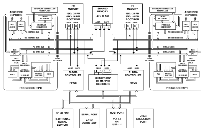
Figure 2. ADSP-2192 Dual-Core DSP Block Diagram
